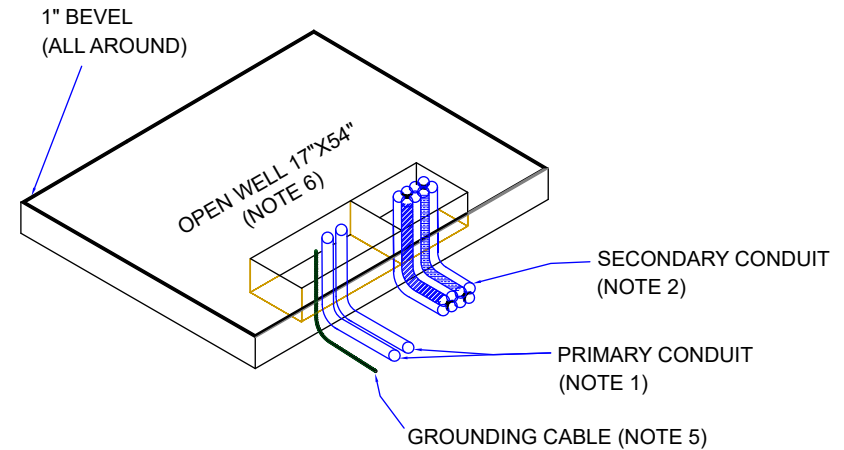
ISOMETRIC VIEW
