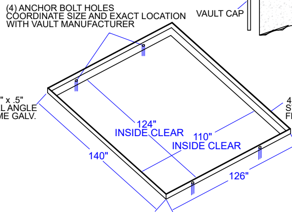
ANGLE SUPPORT FRAME (ANGLE UP)
