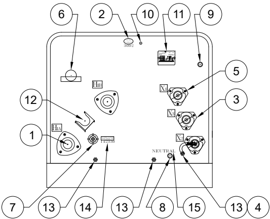
FRONT VIEW 25-100kVA
