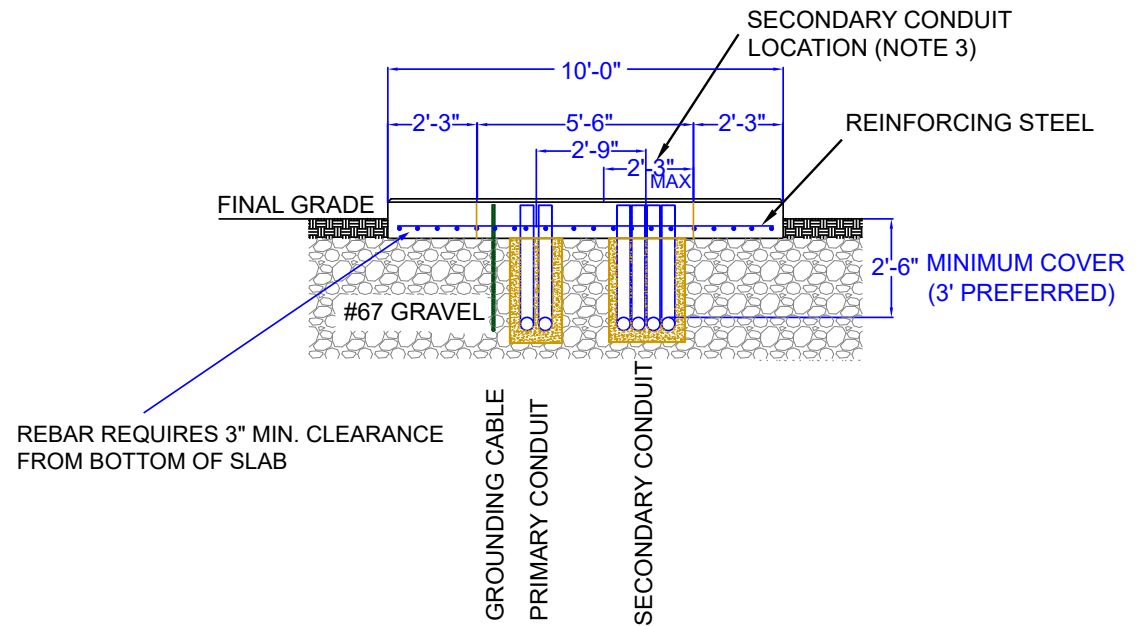
FRONT VIEW
