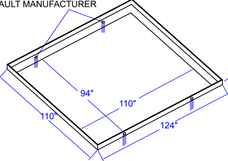
ANGLE SUPPORT FRAME (ANGLE UP)
