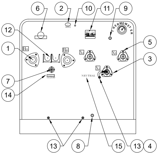
FRONT VIEW 167-250kVA
