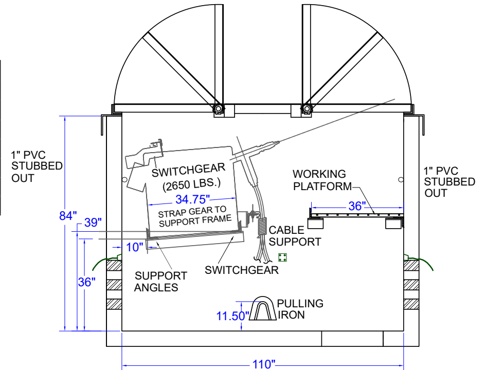
END VIEW
