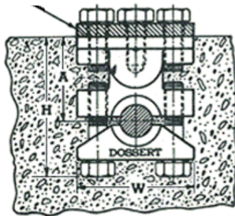
FLAT BUS BAR
