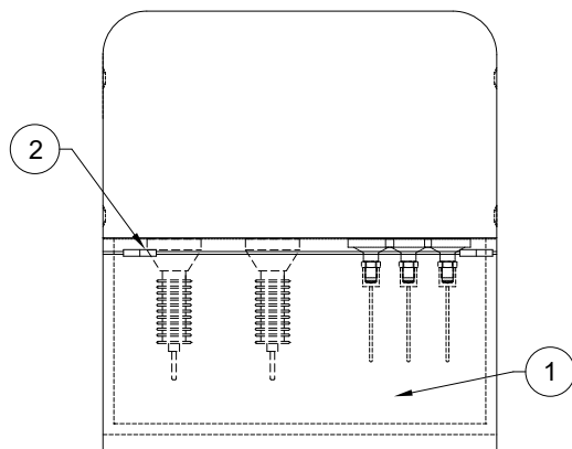
TOP VIEW 25-250kVA
