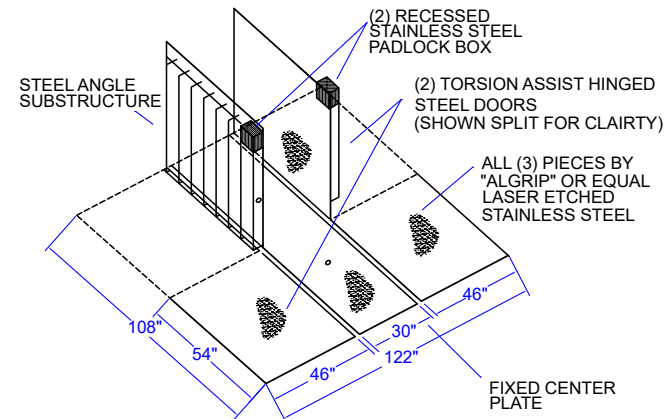
DOORS
