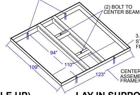
LAY IN SUPPORT FRAME
