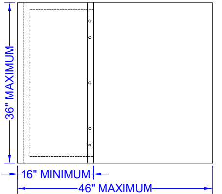
LIMITING DIMENSIONS
