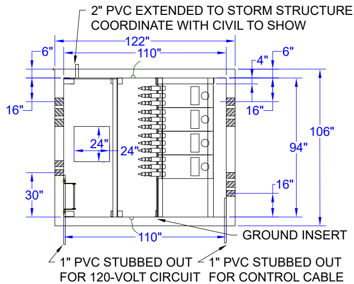
FLOOR PLAN (WORKING PLATFORM NOT SHOWN)
