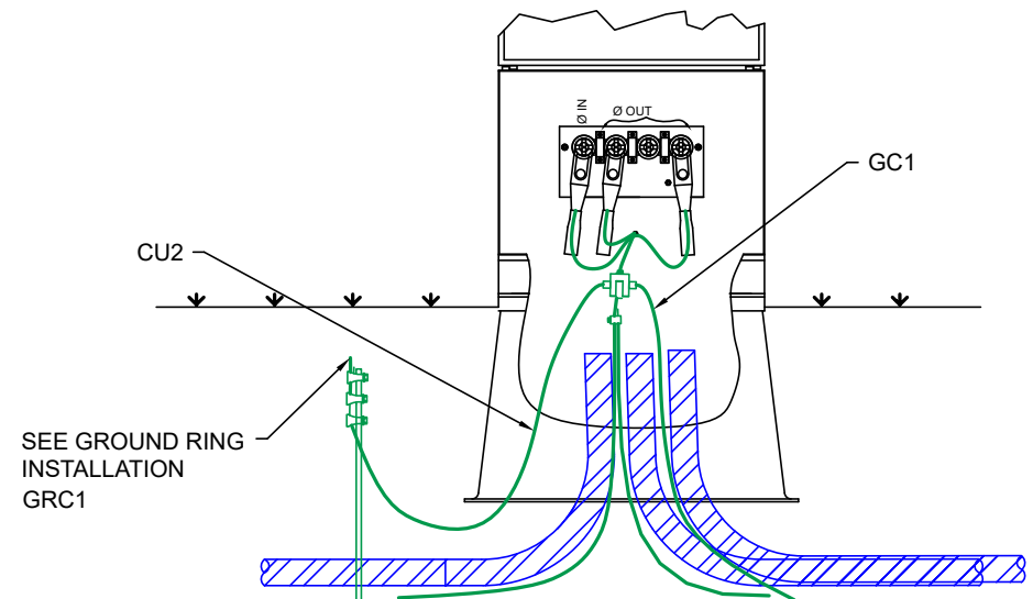
GROUNDING DETAIL
