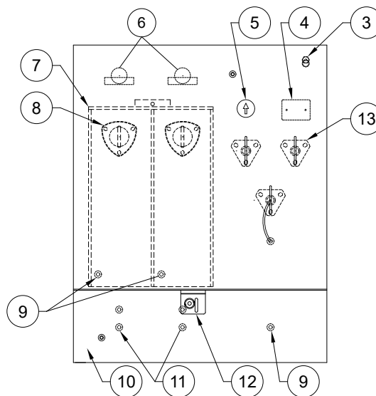
FRONT VIEW 25-250kVA
