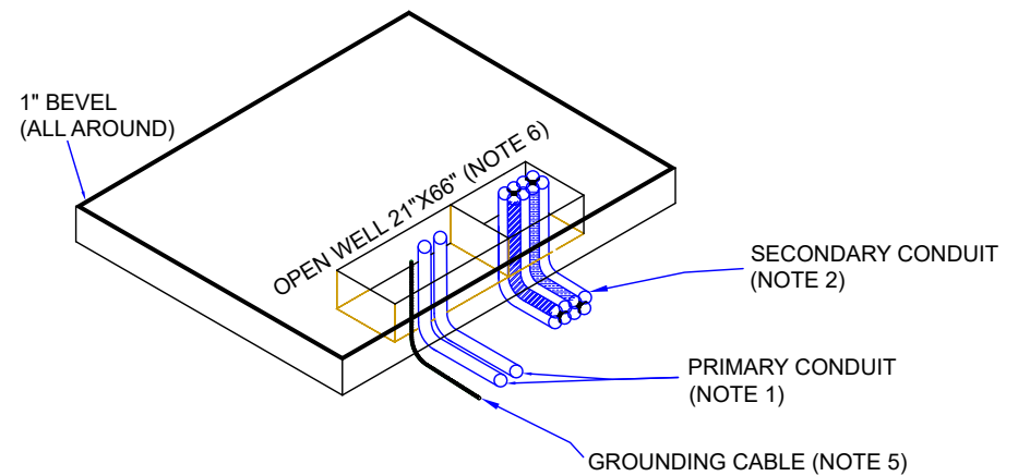
ISOMETRIC VIEW
