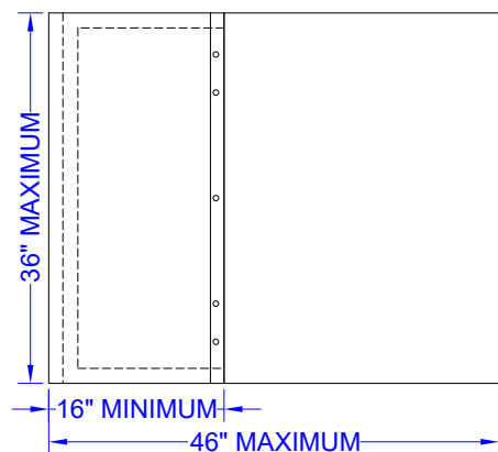
LIMITING DIMENSIONS
